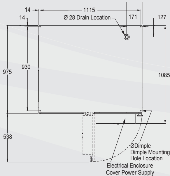
Discharge End
