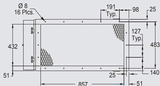
Intake End
