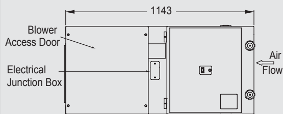
Intake End
